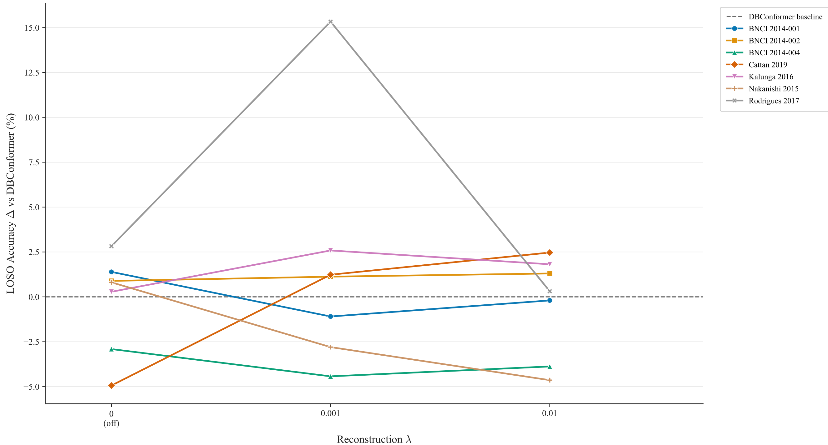
Effect of Reconstruction Weight on Classification Accuracy
